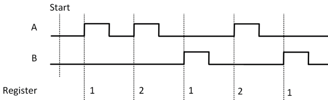
Figure 91 Two-Pulse Encoder in Single Mode
