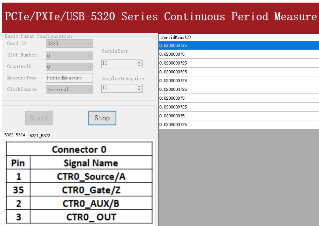
Figure 50 Period Measure For Continuous Mode
