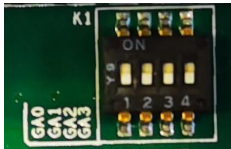
Figure 79 DIP Switch in PCIe-5320
