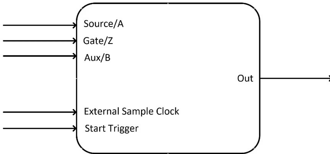
Figure 34 Counter Input Diagram
